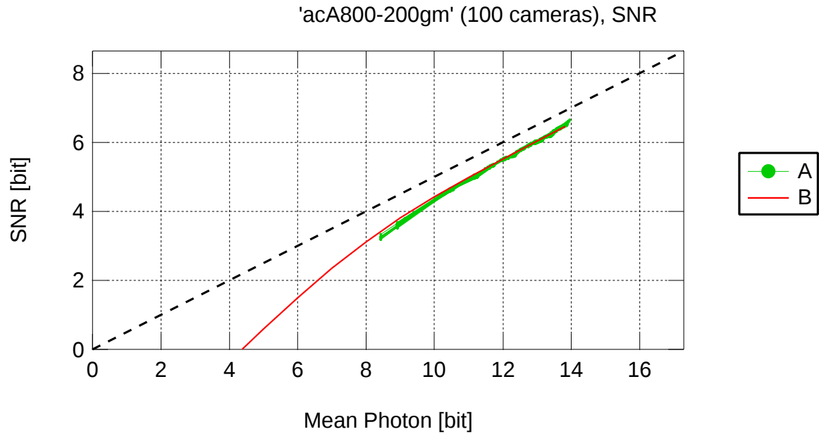
Figure 13: Signal-to-noise Ratio
