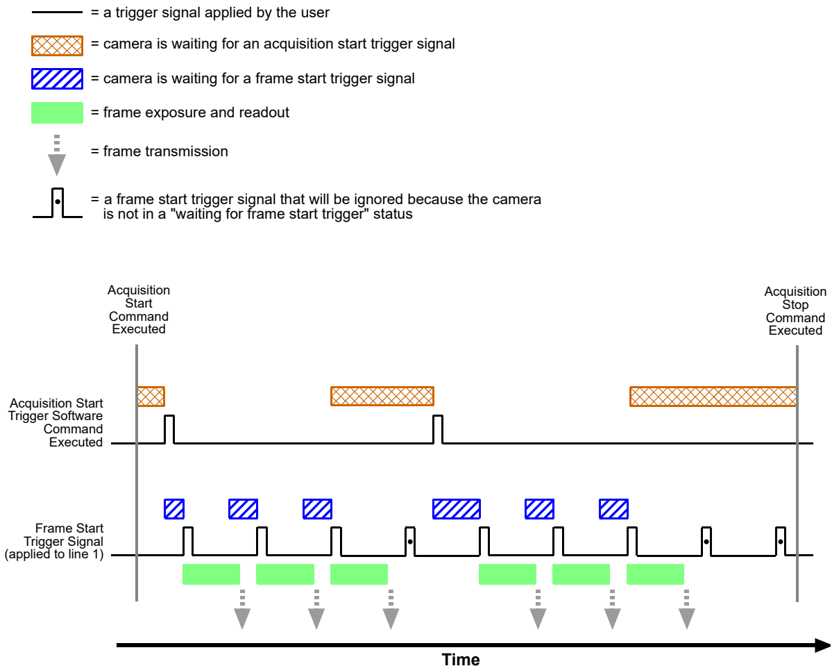
Fig. 35: Use Case 4 - Acquisition Start Trigger On and Frame Start Trigger On
