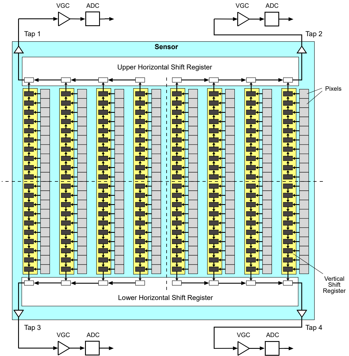
Fig. 7: Four Tap Sensor Readout Mode
