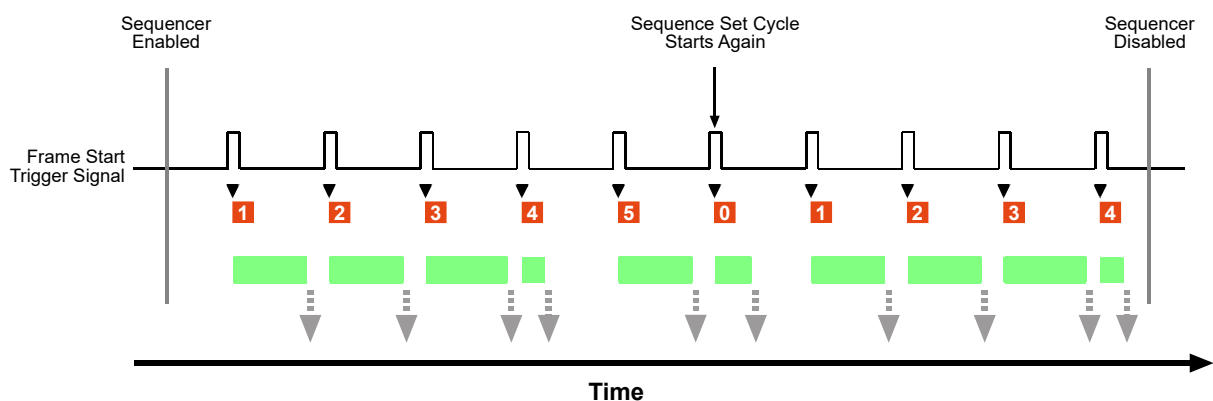
Fig. 47: Sequencer in Controlled Sequence Advance Mode with Always Active as the Sequence Control Source
