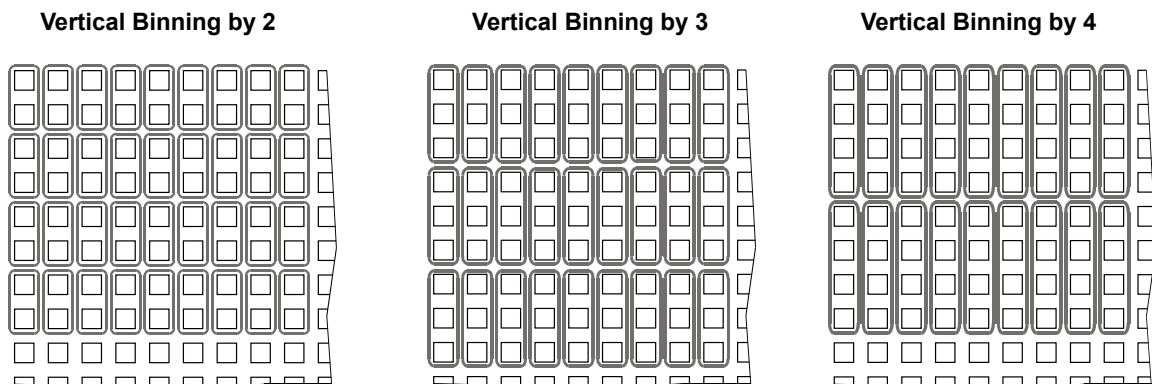
Fig. 53: Vertical Binning
