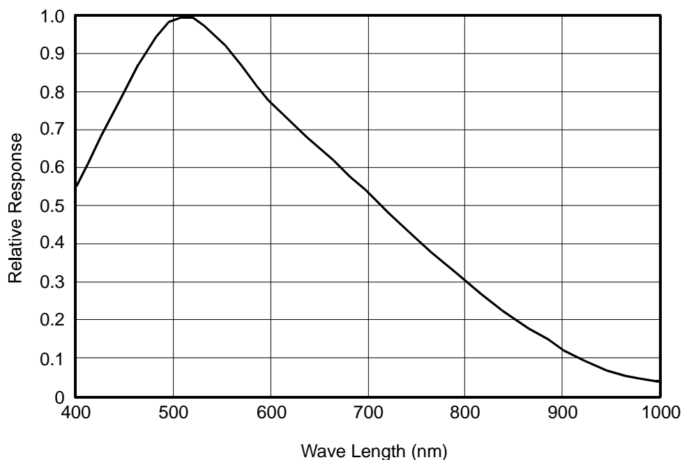
Figure 1-2: A631f Monochrome Camera Spectral Response
