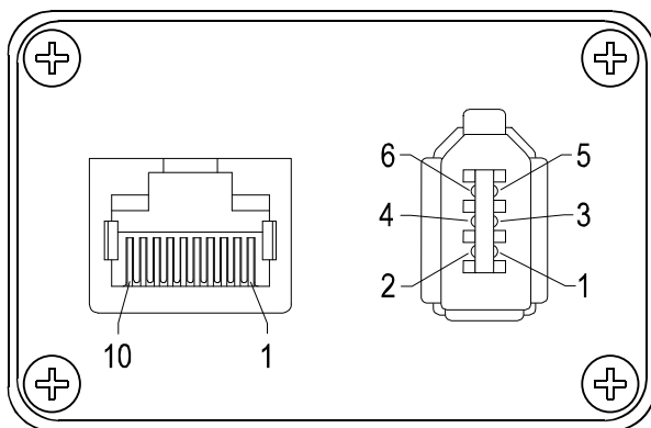
Figure 2-2: A630f Pin Numbering
