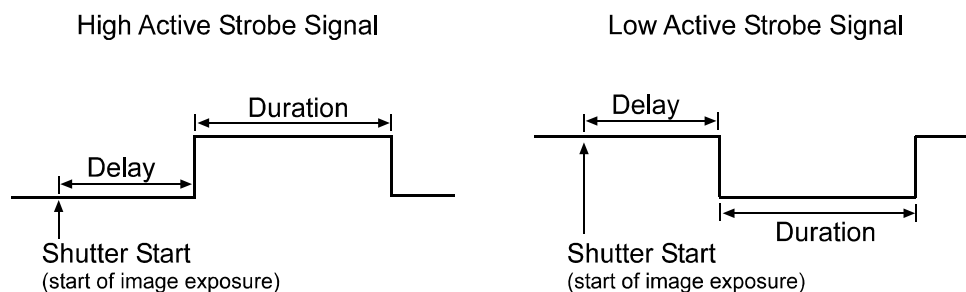
Figure 3-15: Strobe Signal
