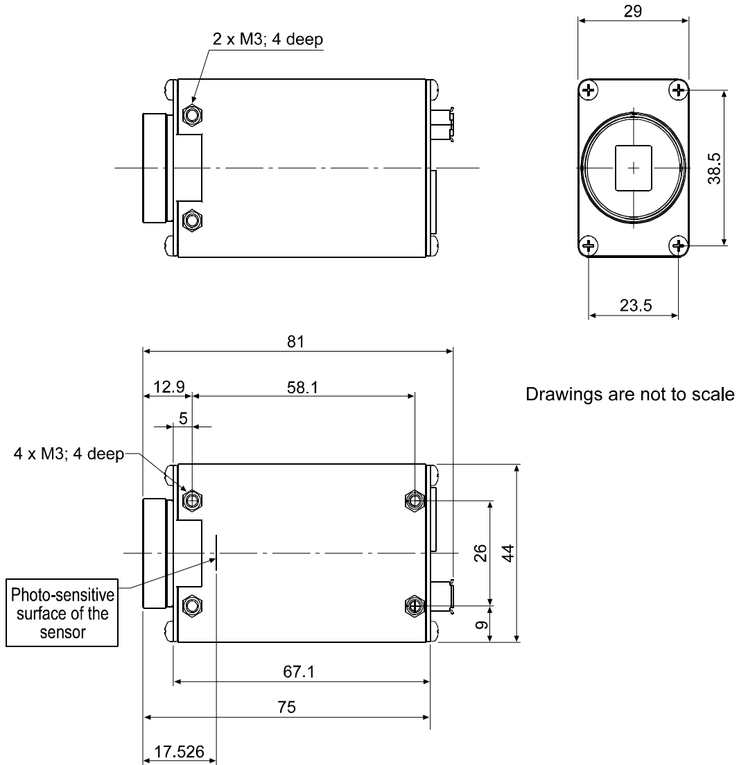
Figure 7-1: A630f Mechanical Dimensions (in mm)
