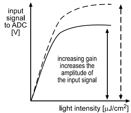
Figure 3-10: Gain
