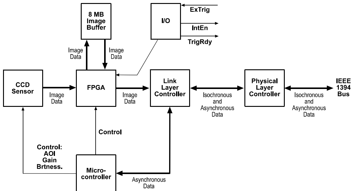
Figure 3-2: A630f Block Diagram
