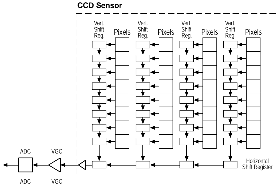
Figure 3-1: A630f Sensor Architecture
