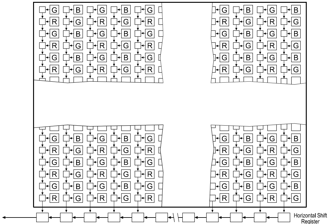
Figure 3-14: Bayer Filter Pattern on the A631fc
