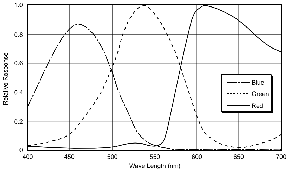
Figure 1-3: A631fc Color Camera Spectral Response
