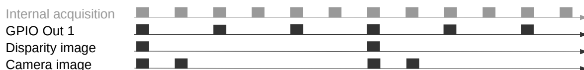
Fig. 6.36: Example of using the ExposureAlternateActive mode for GPIO Out 1 with a user-defined frame rate of 8 Hz. The internal image acquisition is always 25 Hz. GPIO Out 1 is HIGH for the exposure time of every second image. A disparity image is computed for images where Out 1 is HIGH and that are sent out via GigE Vision according to the user-defined frame rate. In ExposureAlternateActive mode, intensity images are always transmitted pairwise: one with GPIO Out 1 HIGH, for which a disparity image might be available, and one with GPIO Out 1 LOW.
